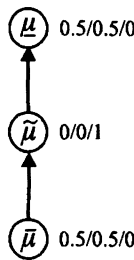
Figure 1. Lattice of Example 3.1
