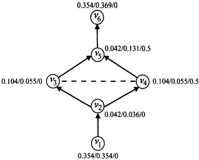
Figure 3. Lattice of Example 3.3
