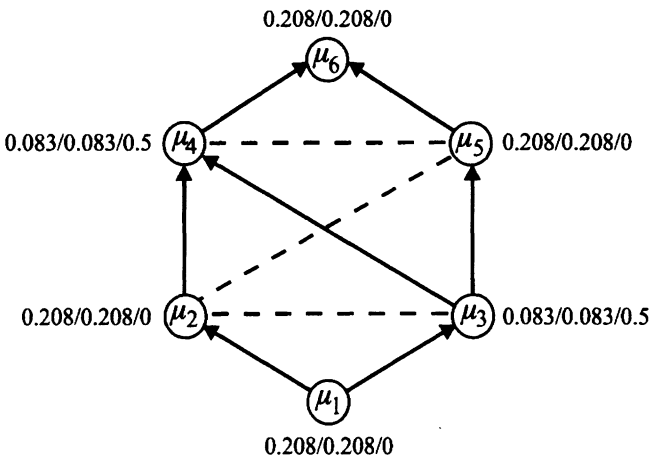
Figure 2. Lattice of Example 3.2
