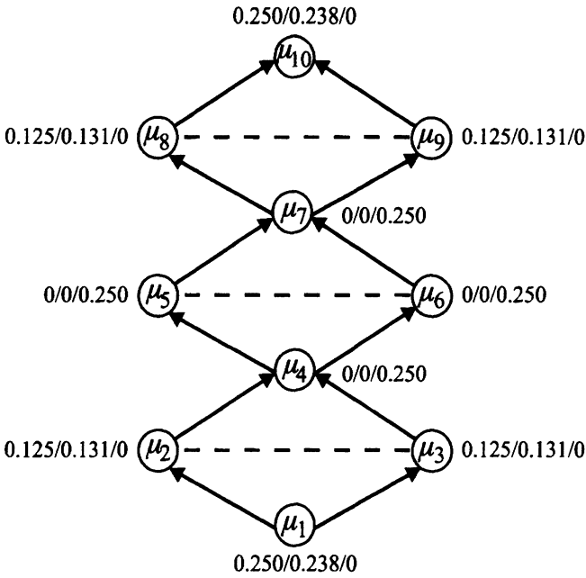
Figure 4. Lattice of Example 3.5
